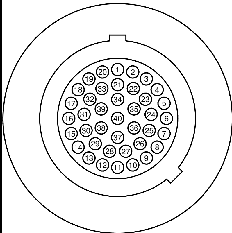
FACE VIEW
