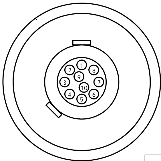
FACE VIEW
