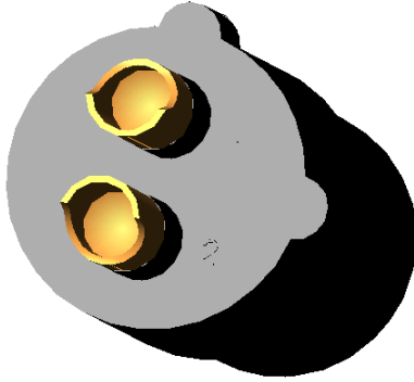
SOLDERPOT VIEW
