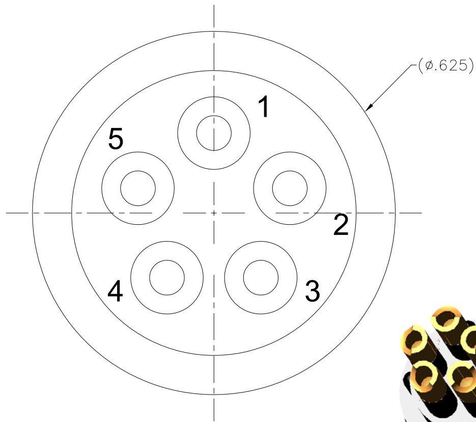
FACE VIEWS
